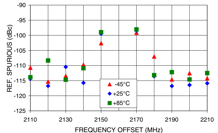
REFERENCE SPURIOUS Vs FREQ. OFFSET @ Fcar = 2160MHz
