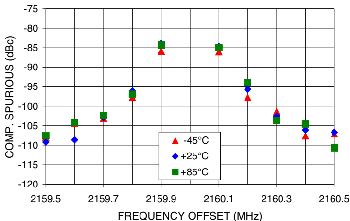
COMPARISON SPURIOUS Vs FREQ. OFFSET @ Fcar = 2160MHz
