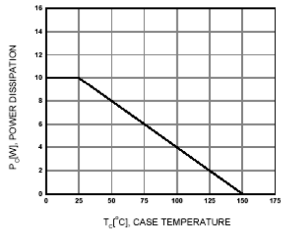
Figure 8. Power Derating
