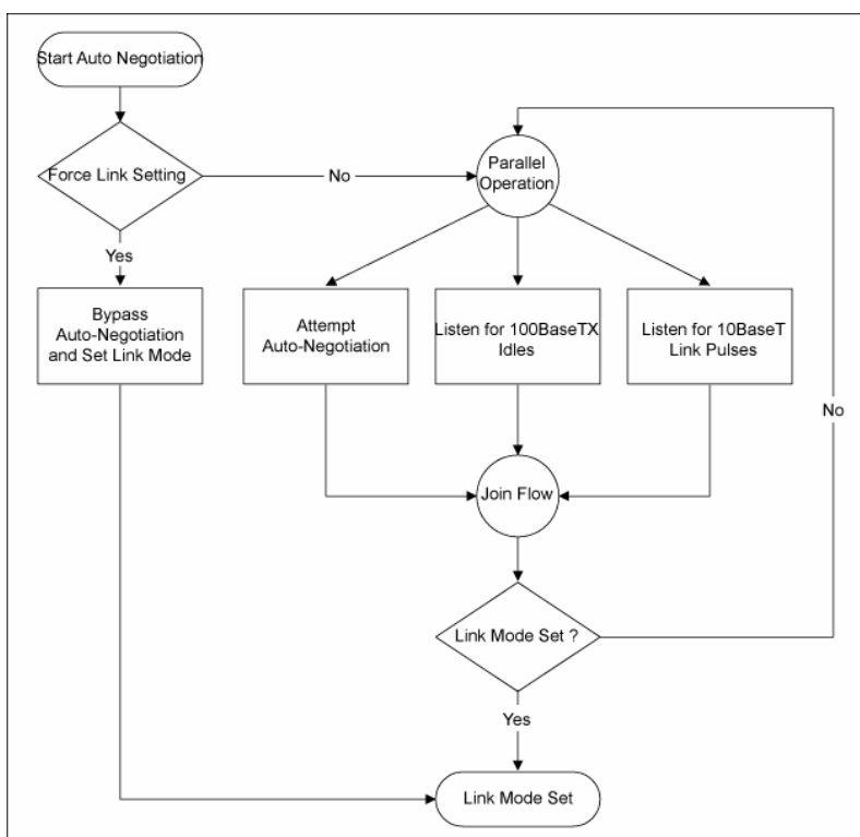
Figure 2. Auto-Negotiation
