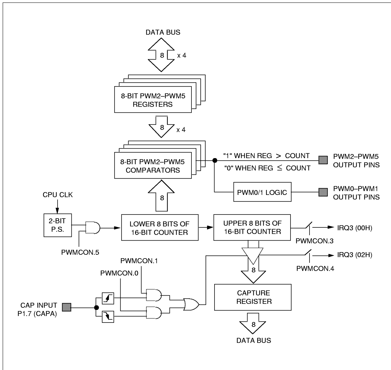
Figure 41. Block Diagram for PWM2–PWM5
