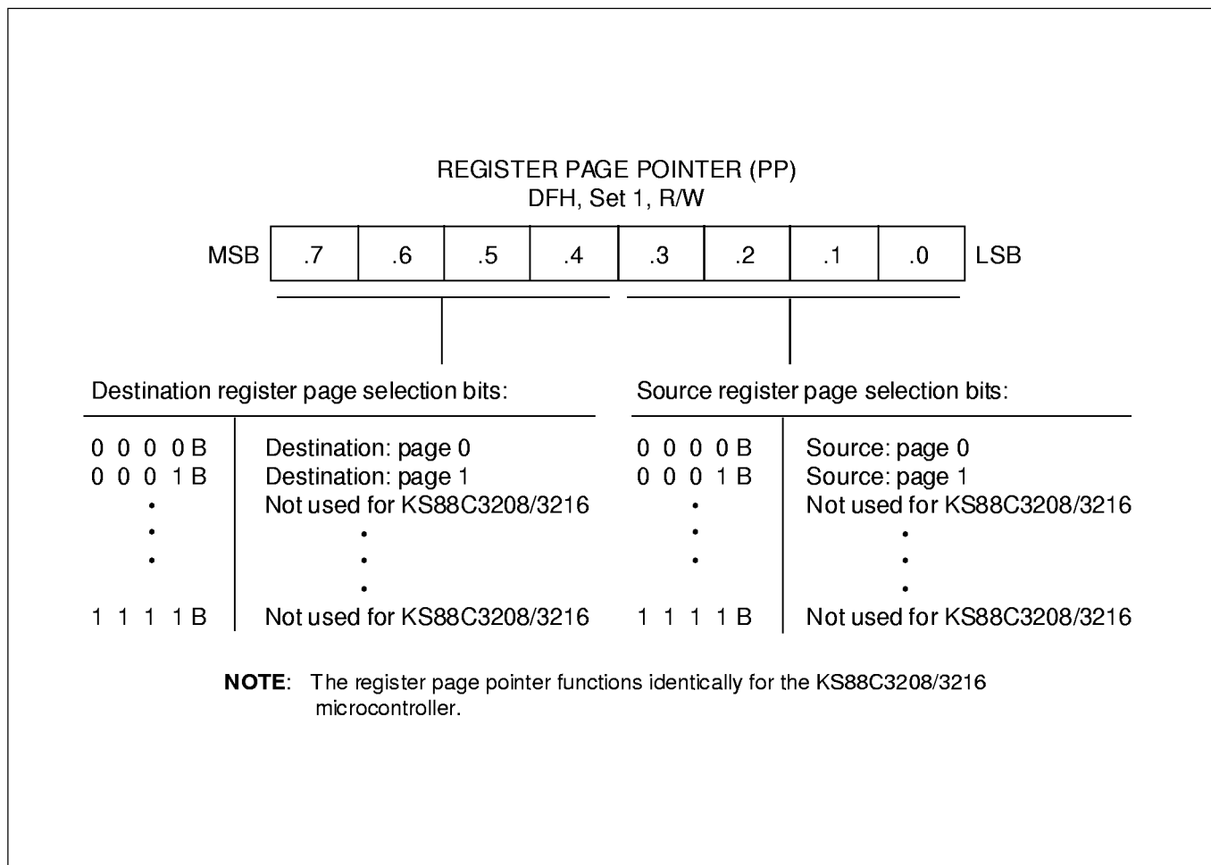
Figure 11. Register Page Pointer (PP)
