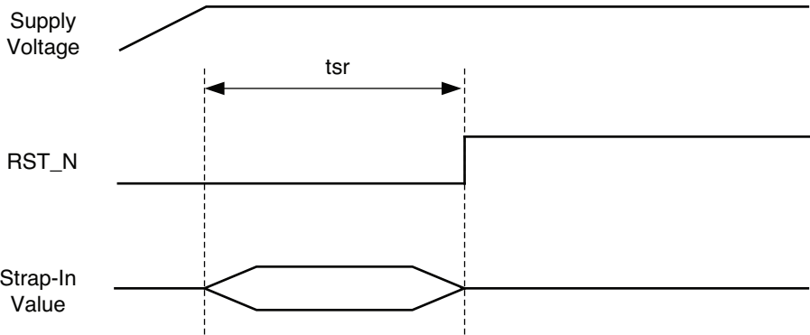
Figure 10. Reset Timing
