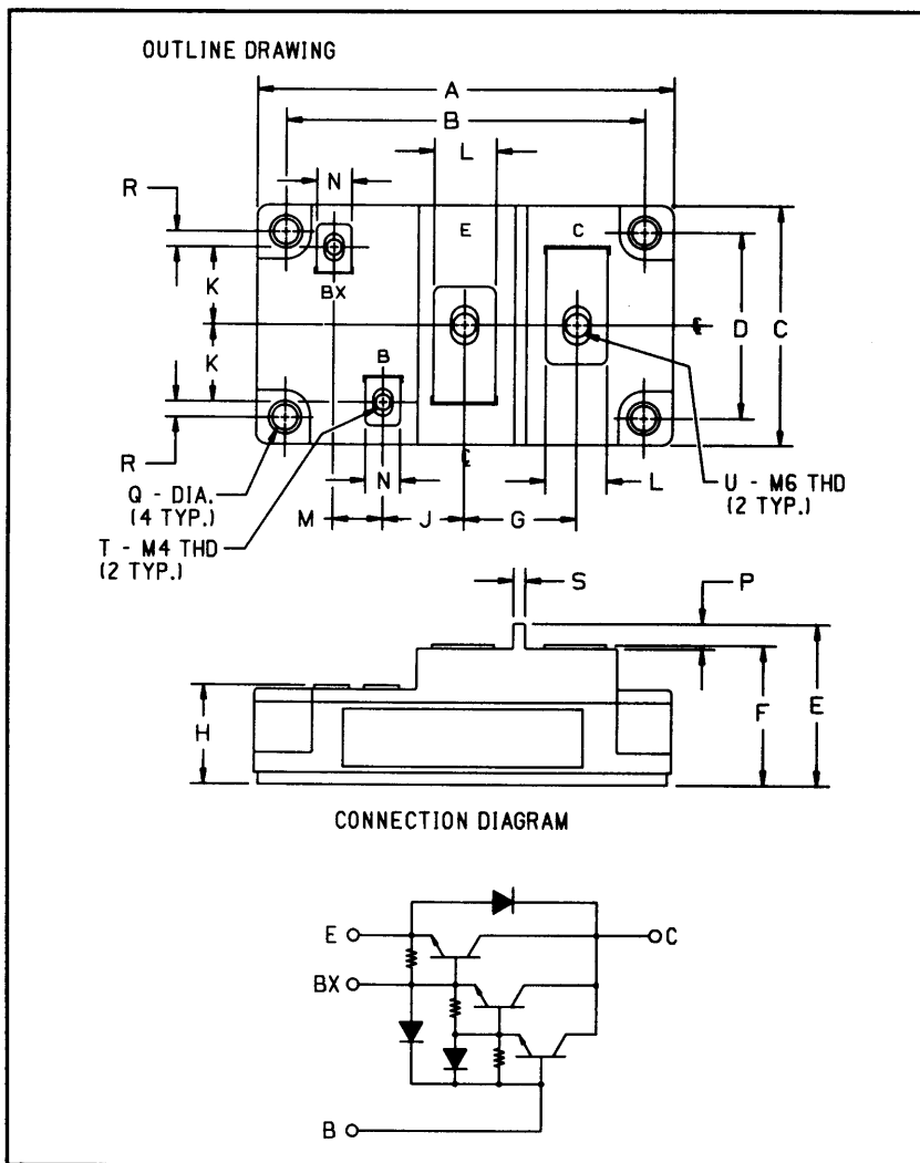
Outline Drawing
