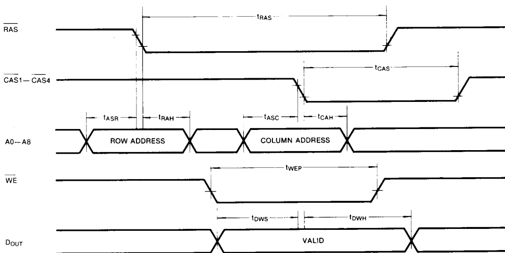
Figure 8. AC Timing Diagrams (1)
