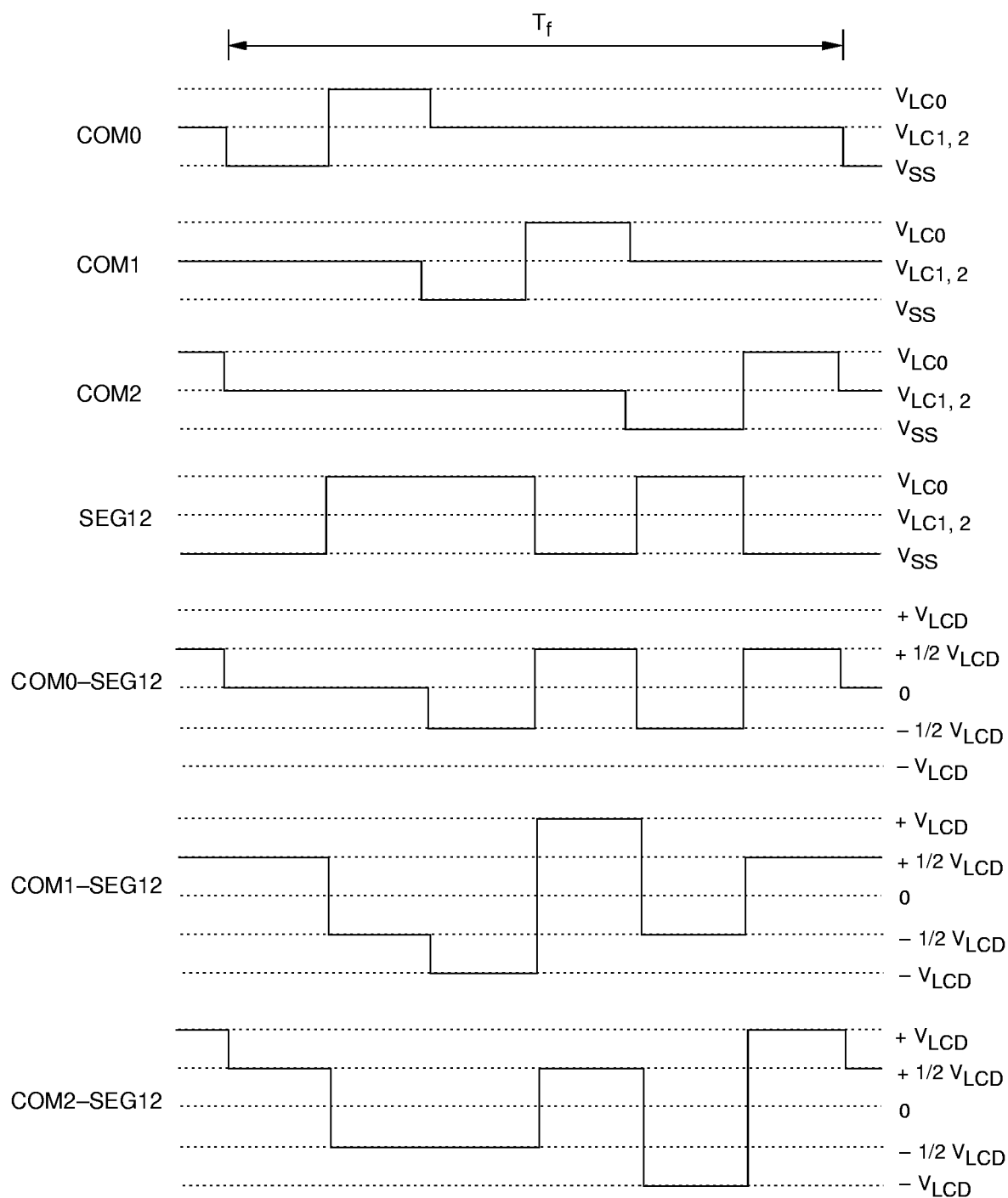
Figure 64. LCD Signal Waveforms at 1/3 Duty, 1/2 Bias
