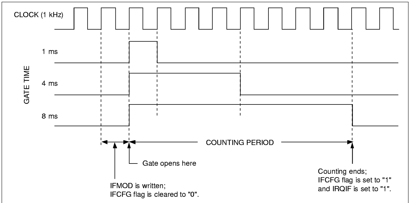
Figure 41. Gate Timing (1, 4, or 8 ms)
