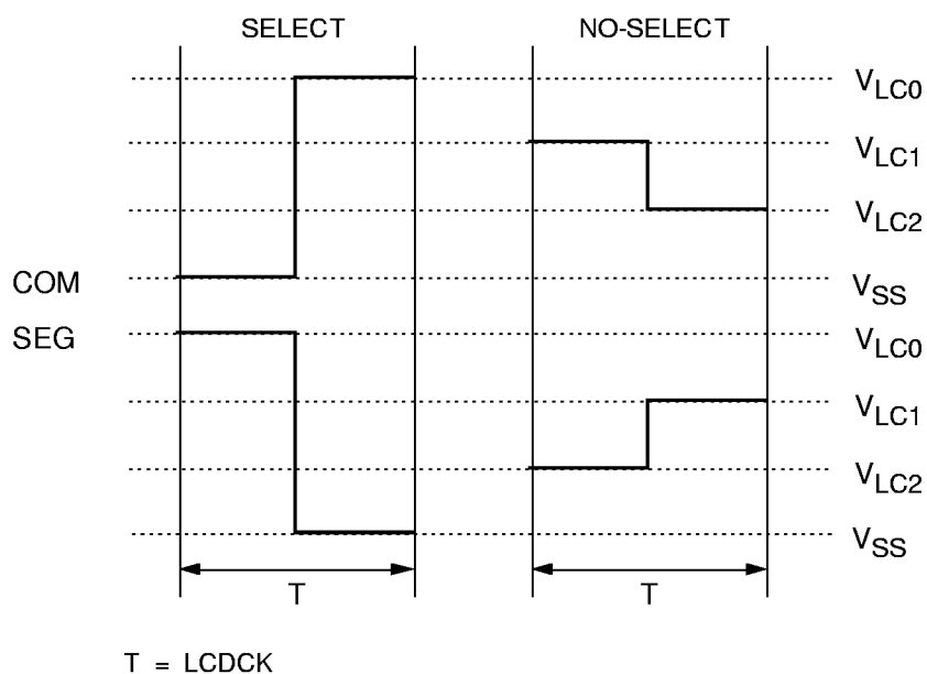
Figure 57. Select/No-Select Signals in 1/3 Bias Display Mode
