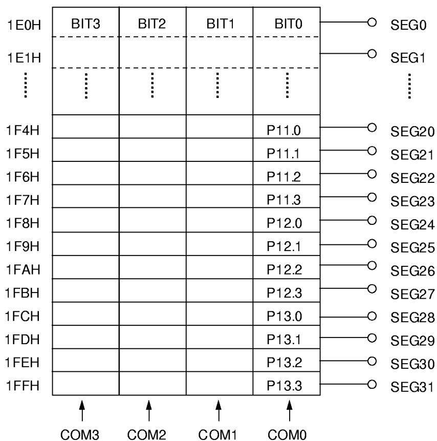
Figure 49. LCD Display Data RAM Organization
