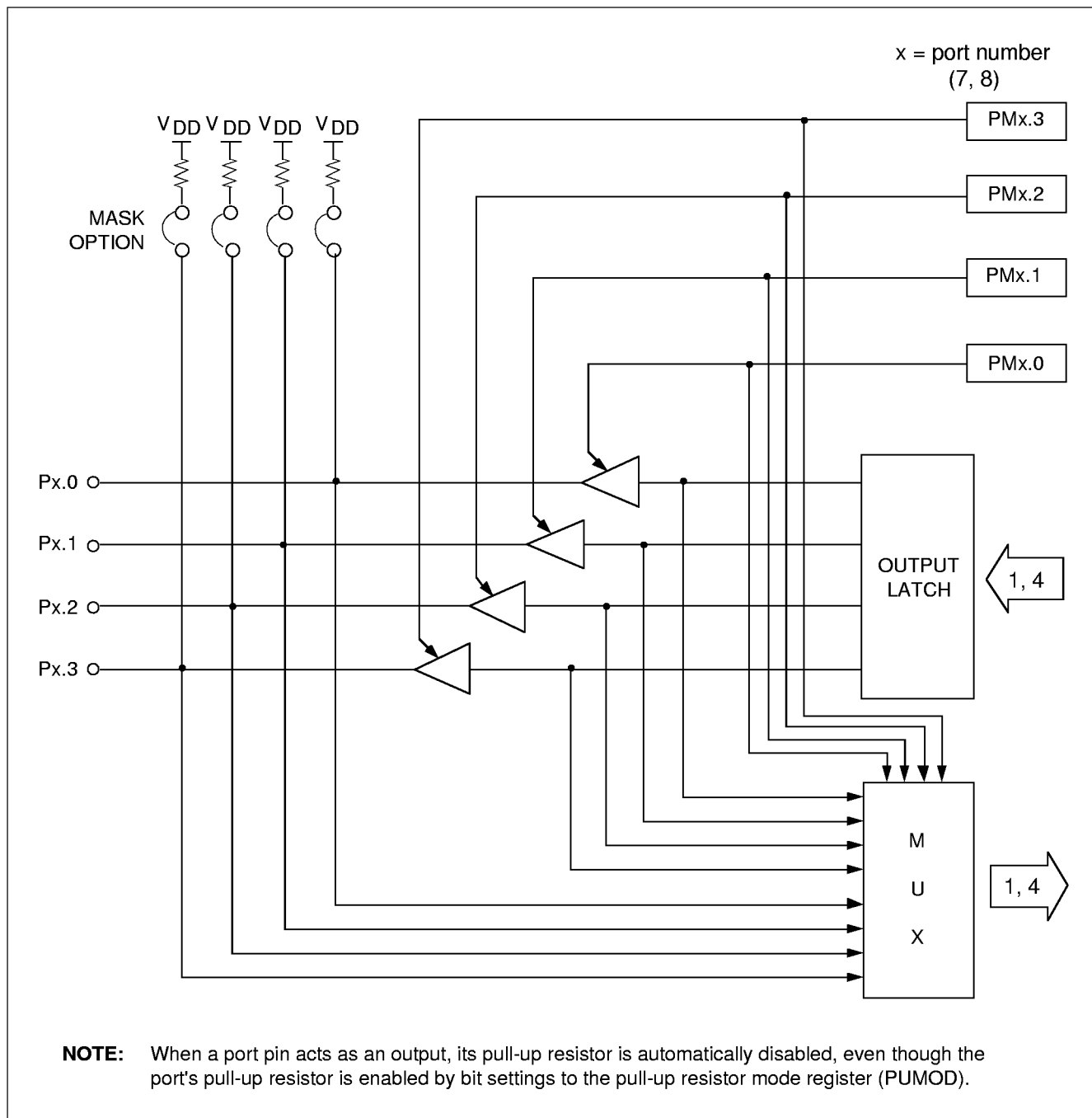
Figure 31. Ports 7 and 8 Circuit Diagram
