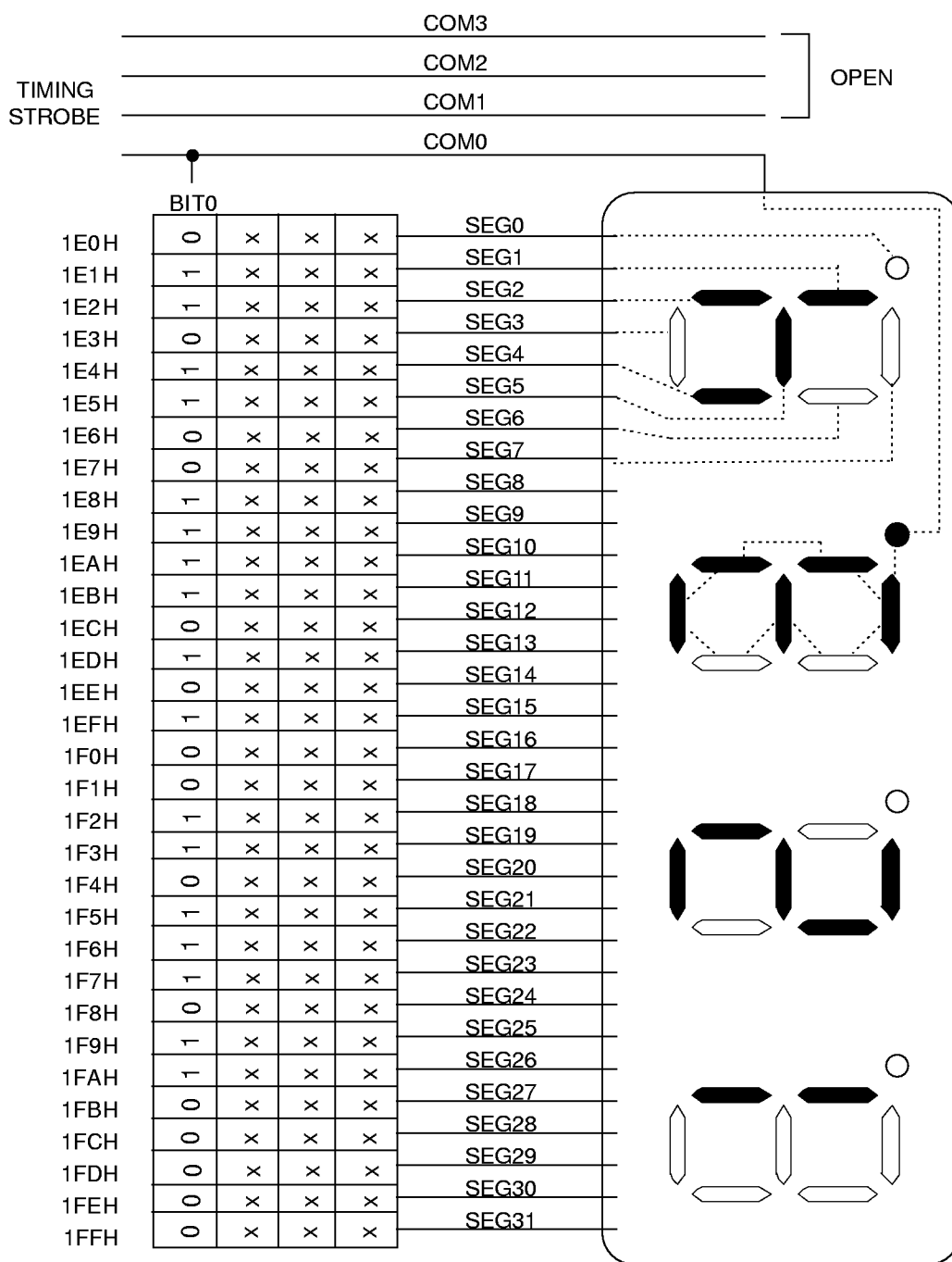
Figure 58. LCD Connection Example (Static)
