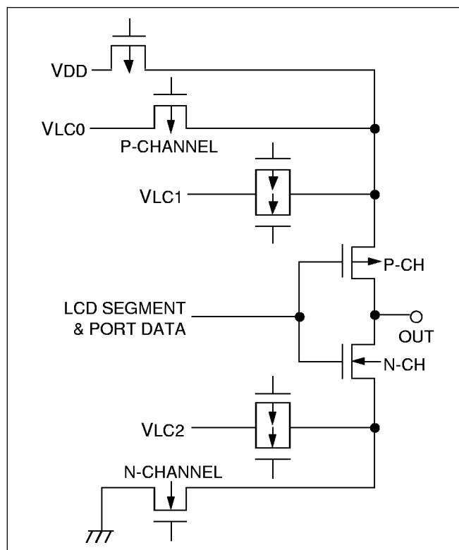
Figure 11. Pin Circuit Type 9
