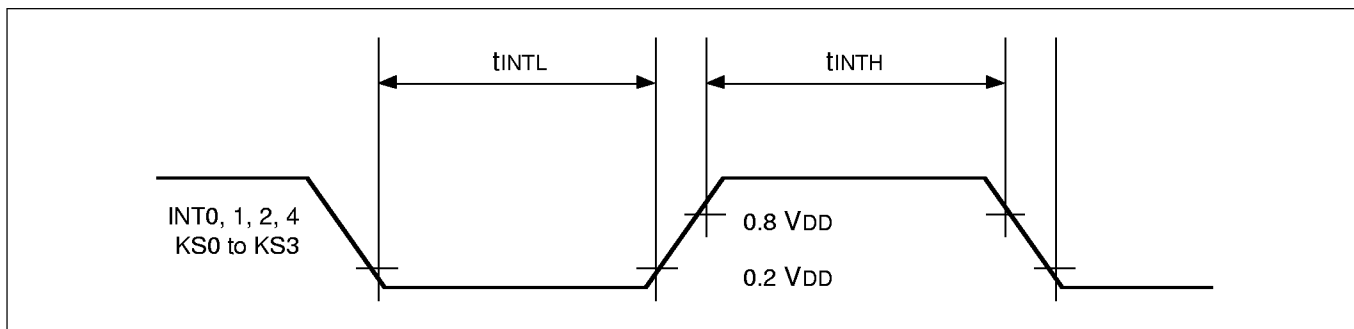
Figure 78. Input Timing for External Interrupts and Quasi-Interrupts
