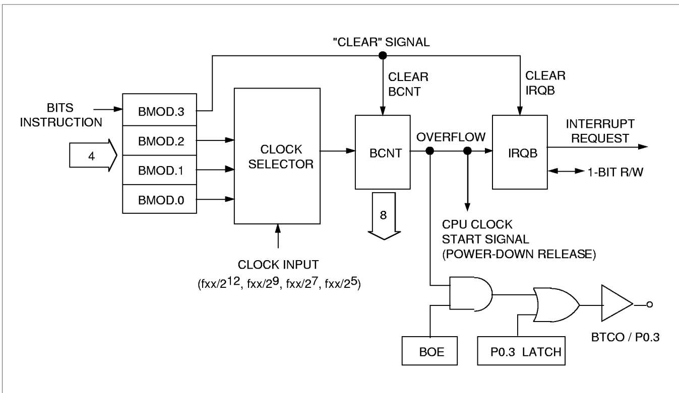
Figure 32. Basic Timer Circuit Diagram
