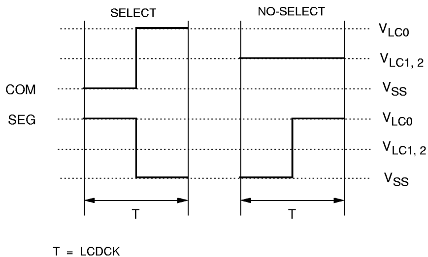
Figure 56. Select/No-Select Bias Signals in 1/2 Bias Display Mode
