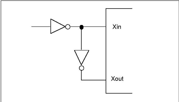
Figure 23. External Oscillator (fx)
