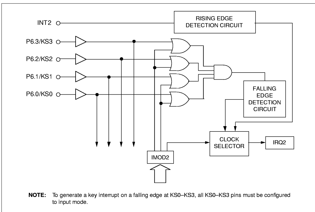
Figure 20. Circuit Diagram for INT2 and KS0-KS3
