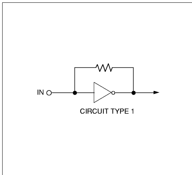
Figure 14. Pin Circuit Type 12
