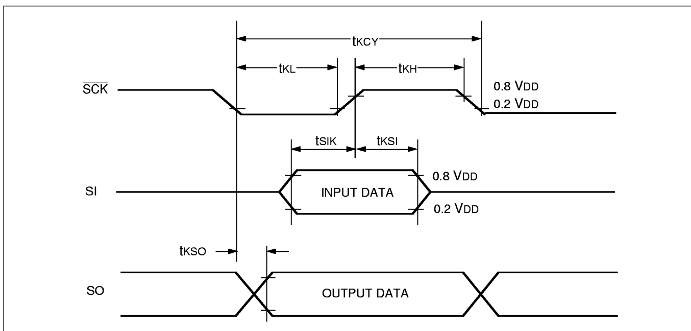
Figure 79. Serial Data Transfer Timing
