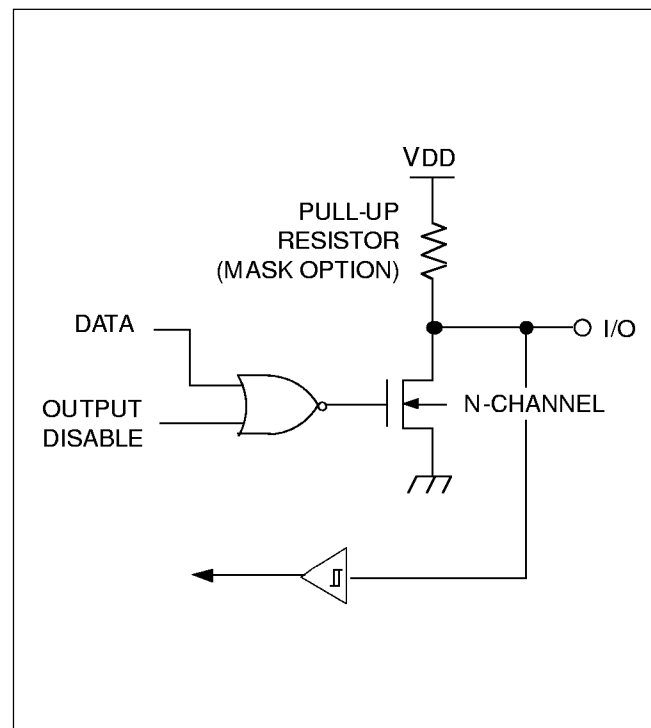
Figure 12. Pin Circuit Type 10
