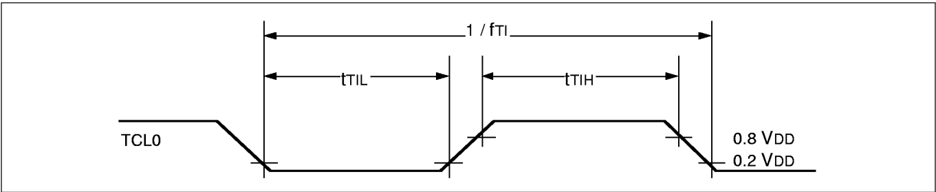
Figure 76. TCL0 Timing
