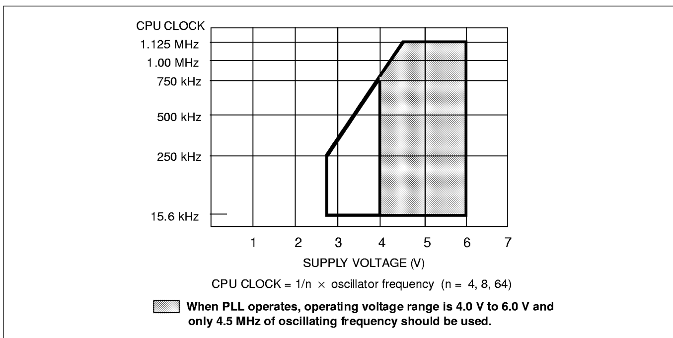
Figure 70. Standard Operating Voltage Range
