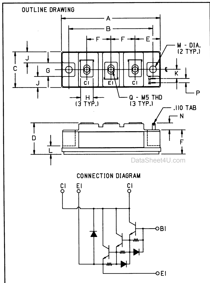
Outline Drawing
