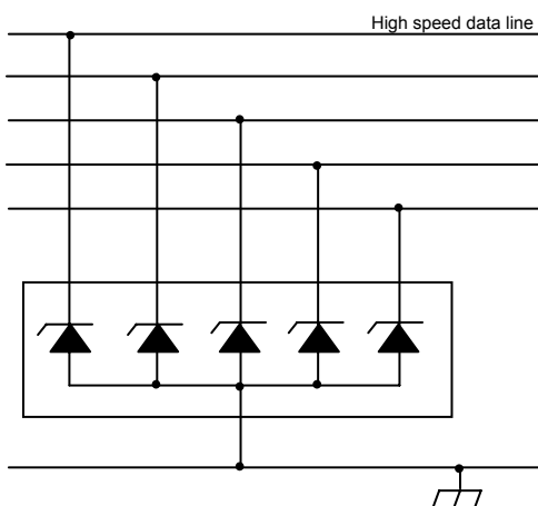
Typical application for uni-directional protection of five lines
