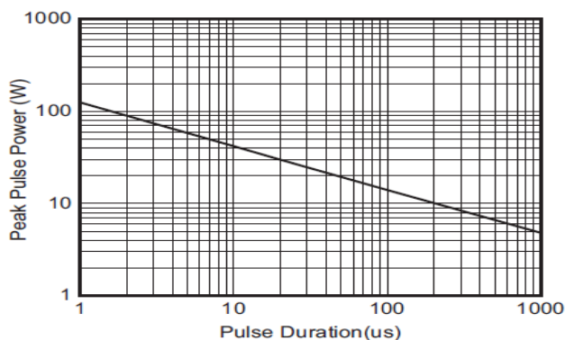
Non-Repetitive Peak Pulse Power vs. Pulse time
