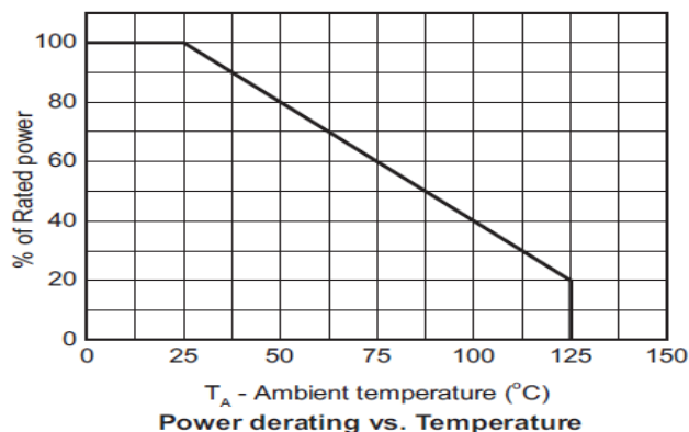
Power derating vs. Temperature
