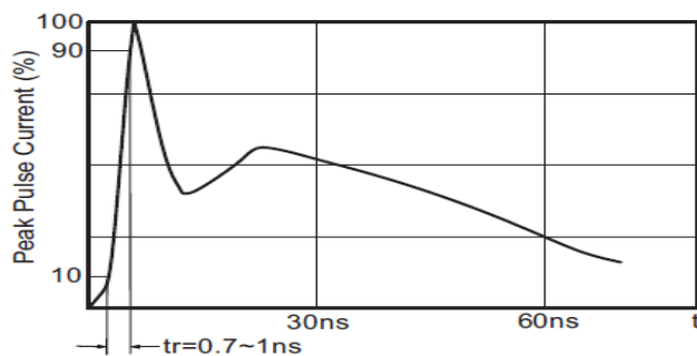
IEC61000-4-2 waveform
