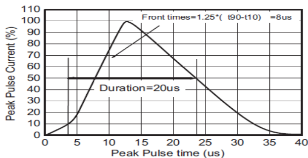
8/20us waveform
