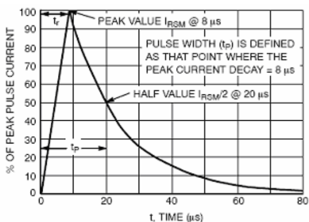
Figure 2. 8 x 20 μs Pulse Waveform
