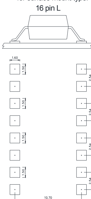
2.Long creepage distance for surface mount type.
