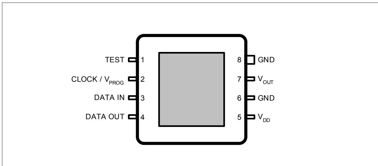
Figure 1 Pin Configuration (top view, figure not to scale)
