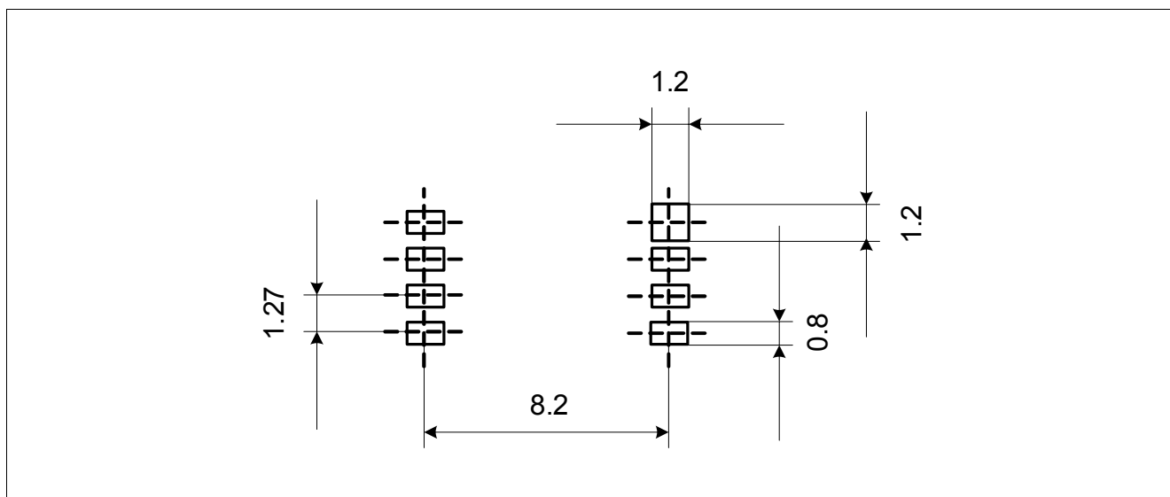
Figure 13 Footprint
