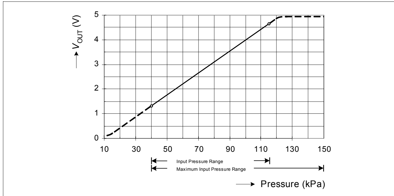
Figure 3 Transfer Function
