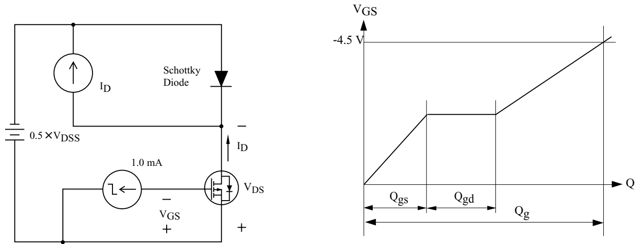
Fig10. Gate Charge
