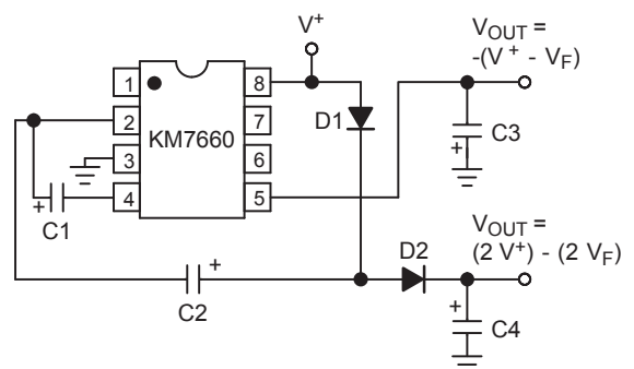
Figure 10. Combined Negative Converter and Positive Multiplier
