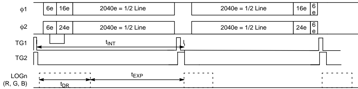
Figure 16. Line Timing
