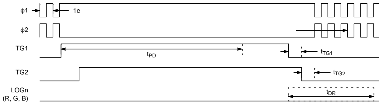
Figure 17. Photodiode-to-CCD Transfer
