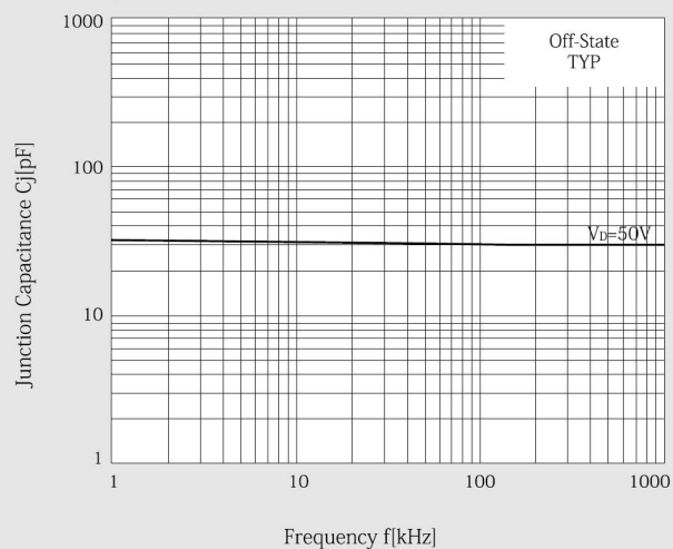
Junction Capacitance
