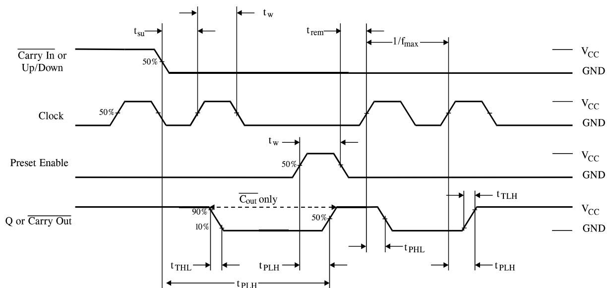
Figure 1. Switching Waveforms
