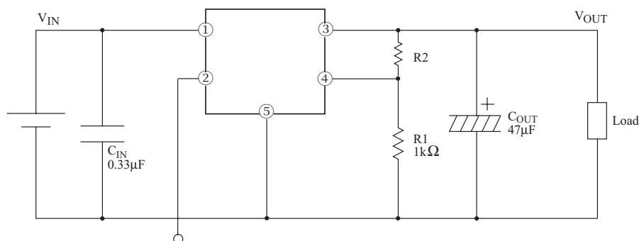
Fig. 6 Application Circuit (Adjustable - Type)
