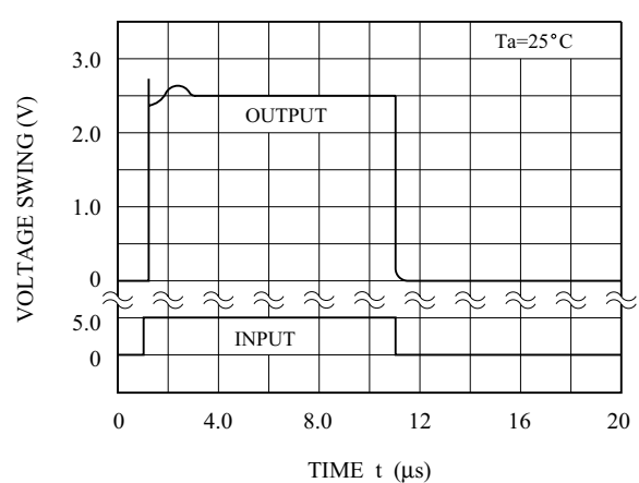
PULSE RESPONSE
