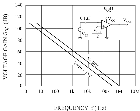
G_V - f
