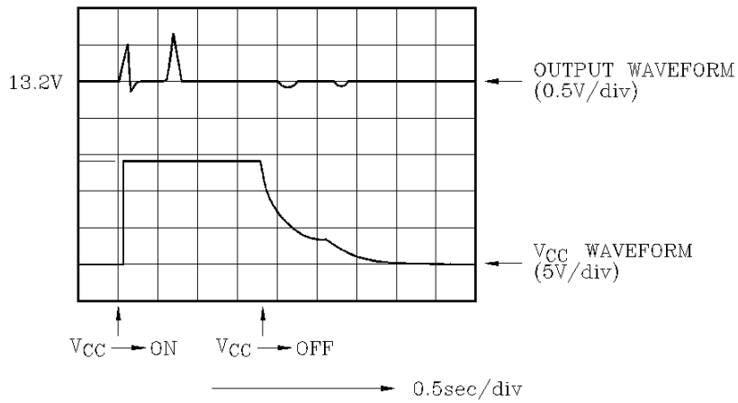
Fig. 6 DUAL OPERATION
