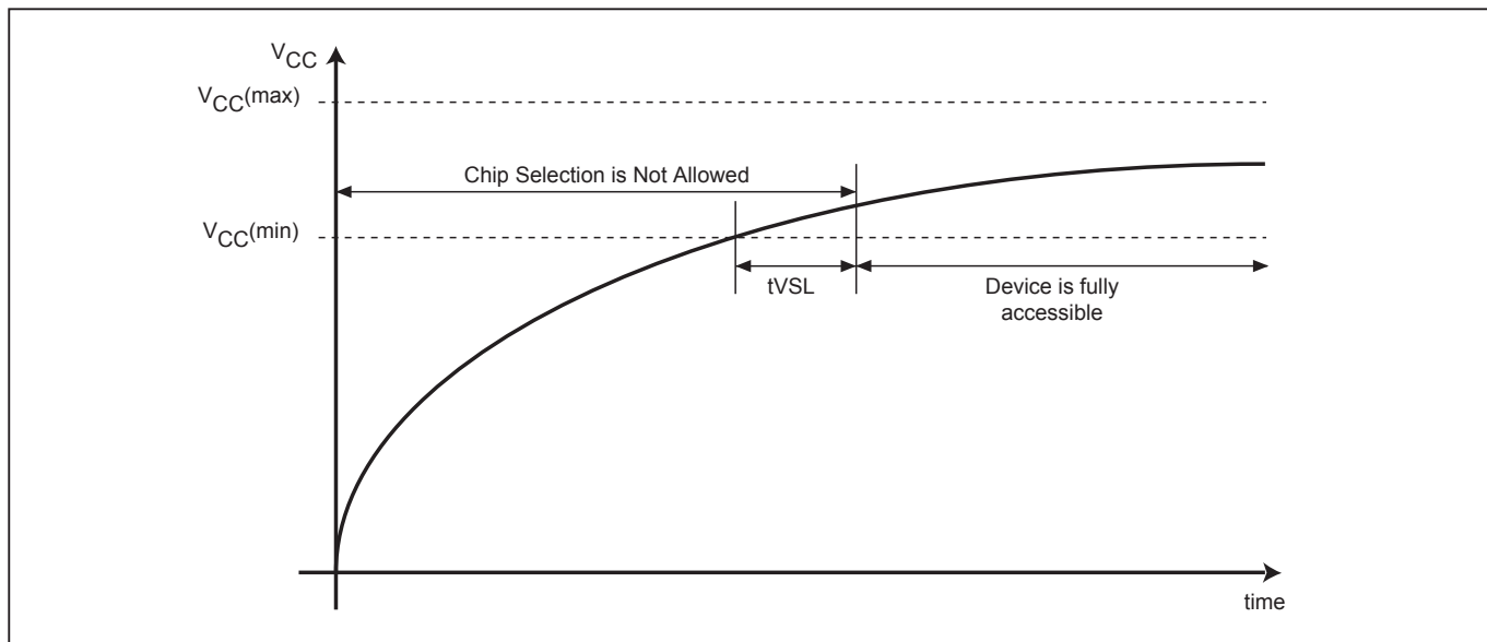
Figure 26. Power-Up Timing
