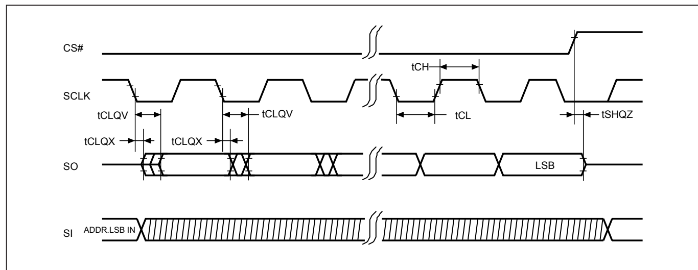
Figure 9. Output Timing
