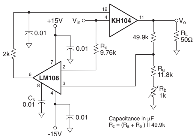
If lower offset and offset drift are required, a low frequency op amp may be used in conjunction with the KH104 in a composite configuration. The suggested circuit appears in Figure 2. Its method of operation is to compare an attenuated version of the output signal to the input signal and apply a correcting voltage at the offset adjust pin. A compensation capacitor C_s reduces the bandwidth of the op amp correction circuit to limit the op amp's effect on the KH104 to frequencies below f_{45} , the frequency at which the op amp has 45dB of open loop gain. Using an LM108, f_{45} is about 7Hz with C_s = 0.1\mu\text{F} . Thus the op amp can correct DC and low frequency errors below f_{45} , without affecting KH104 performance above f_{45} . Also note that the noise performance of the op amp will dominate below f_{45} .
