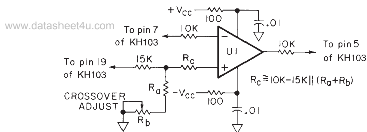
Figure 3: Non-Inverting Gain Composite Amplifier to be Used with Figure 1 Circuit
