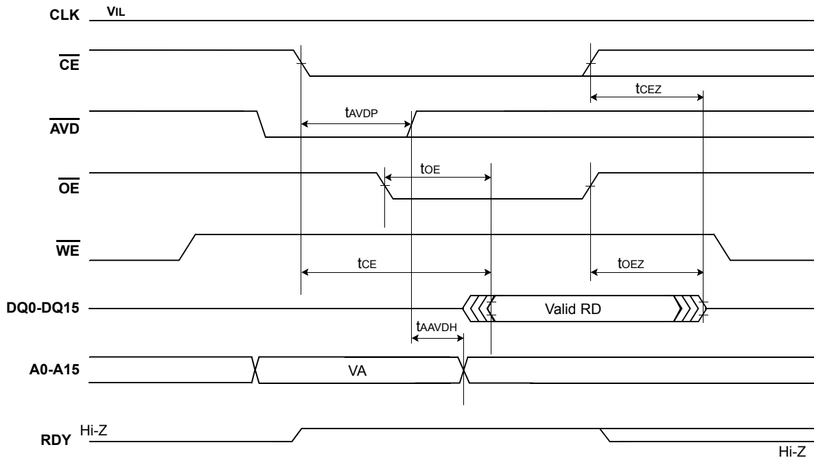
Figure 30. Asynchronous Read Mode( \overline{\text{AVD}} toggling)
