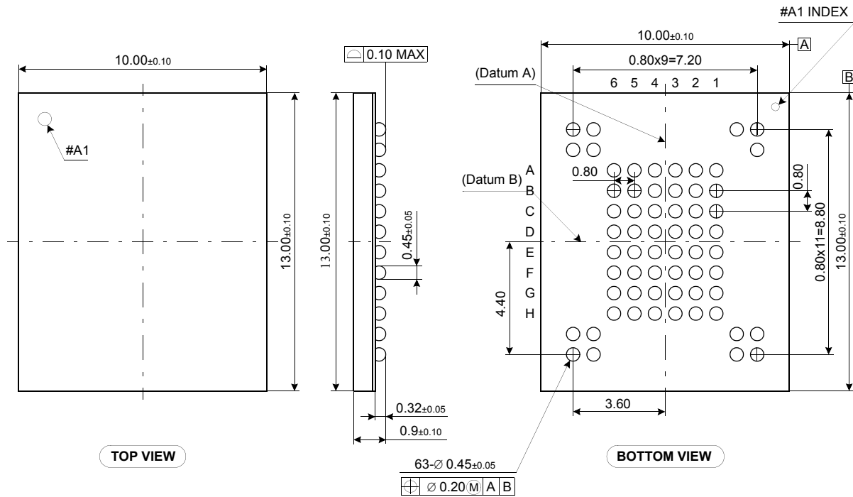
1Gb product (KFG1G16x2B)
