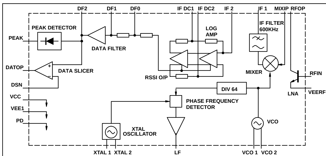
Fig. 2. Block diagram
