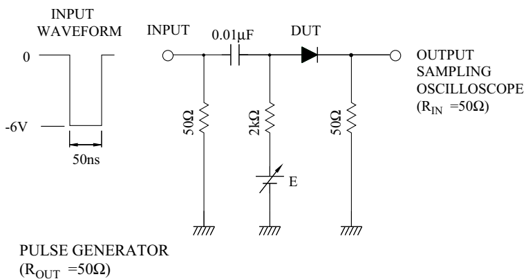
Fig. 1. REVERSE RECOVERY TIME( t_{rr} ) TEST CIRCUIT
