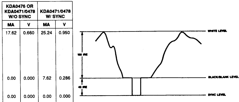
Figure 2. Composite Video Output Waveforms (SETUP = GND)
