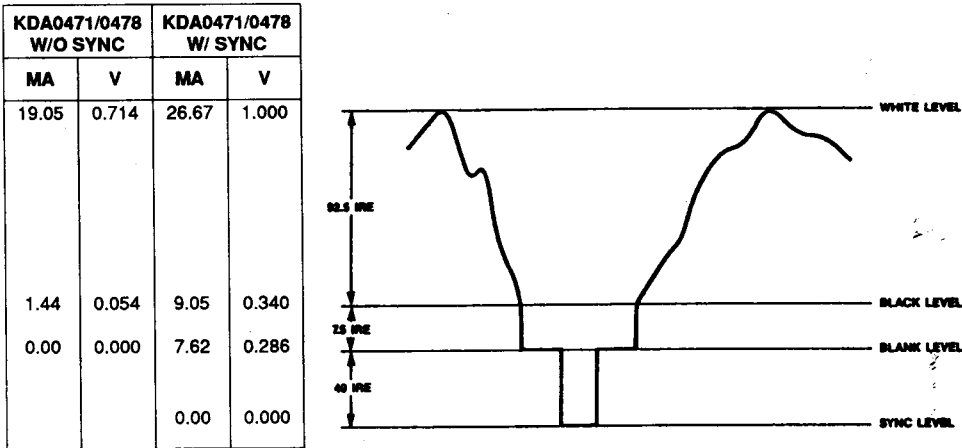
Figure 1. Composite Video Output Waveforms (SETUP = V AA )
