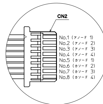
DETAIL B (5:1)
