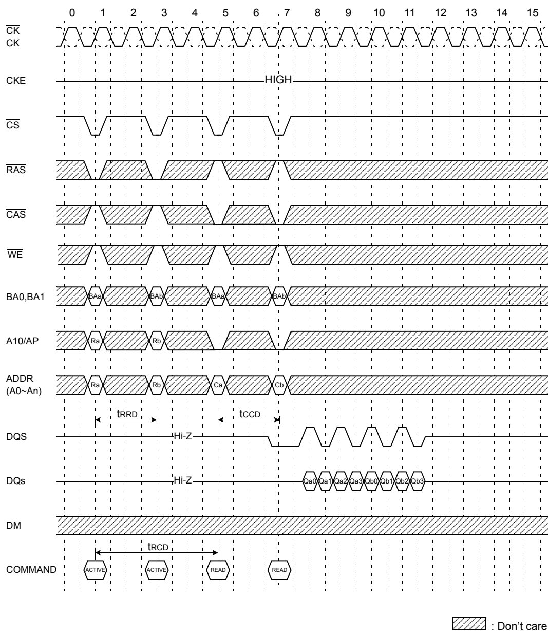
Figure 20. Multi Bank Interleaving READ (@BL=4, CL=3)
