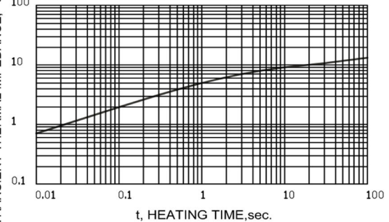
FIG.6-TYPICAL TRANSIENT THERMAL IMPEDANCE PER LEG
