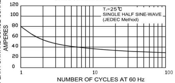
FIG.2-MAXIMUM NON-REPETITIVE PEAK FORWARD SURGE CURRENT PER LEG
