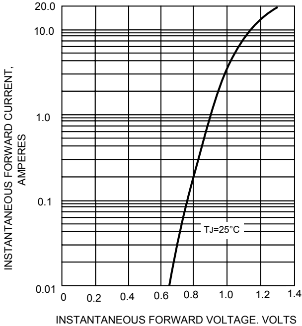
FIG.2-TYPICAL FORWARD CHARACTERISTICS
