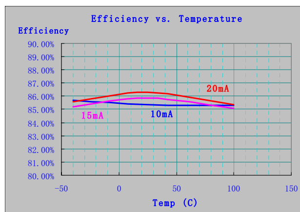
Figure 4. Efficiency vs Temperature
