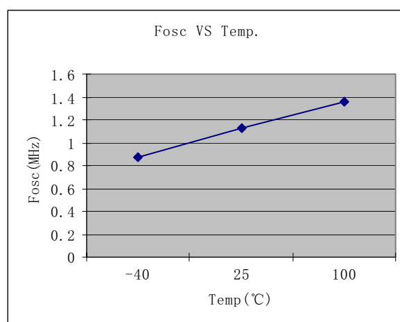
Figure 6. Fosc vs. Temperature
