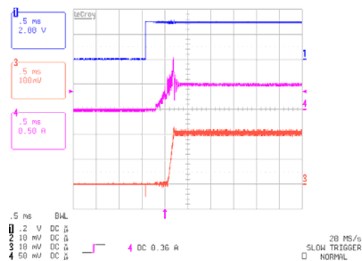
Start-Up Waveform
