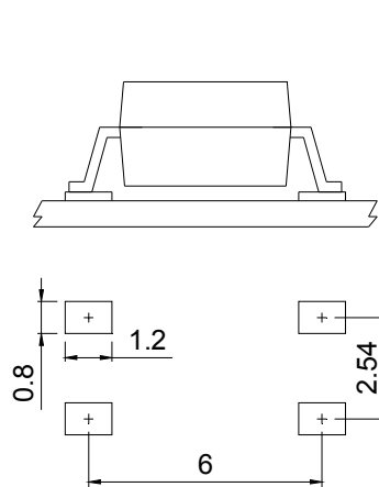
4-pin SOP
