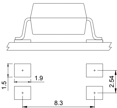
4-pin SMD
