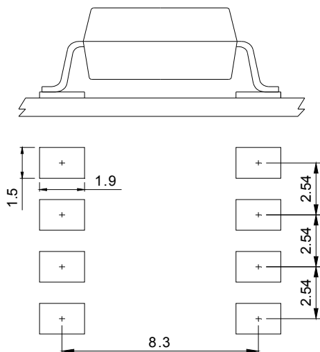
8-pin SMD
