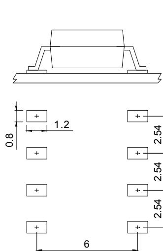
8-pin SOP
