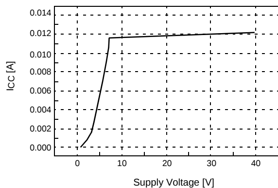
Figure 3. Vcc-Icc
