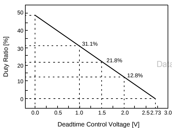
Figure 5. PIN19(Dead Time Control Voltage)-Duty Cycle
