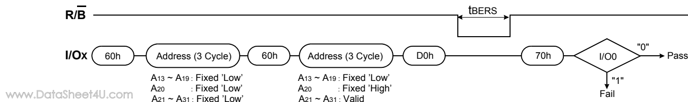
Figure 17. Two-Plane Erase Operation
