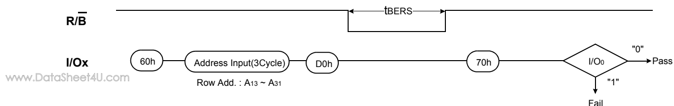
Figure 12. Block Erase Operation
