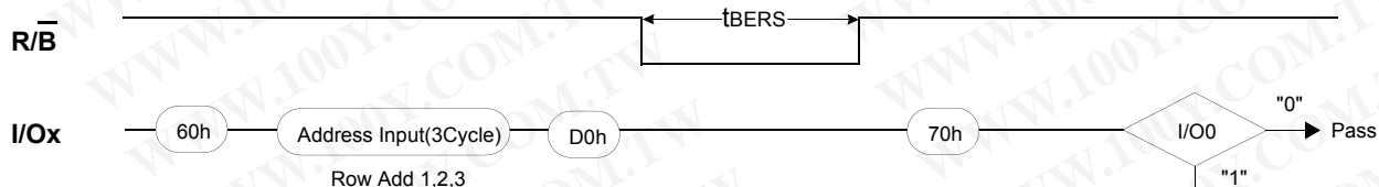
Figure 20. Block Erase Operation
