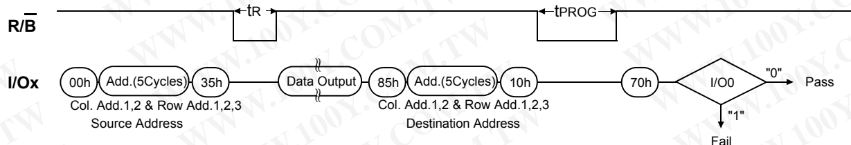
Figure 13. Page Copy-Back Program Operation
