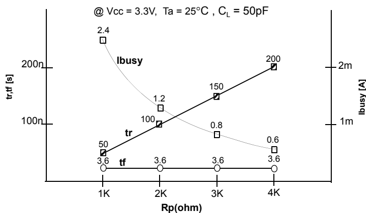
Figure 15. R_p vs t_r , t_f & R_p vs i_{\text{busy}}
