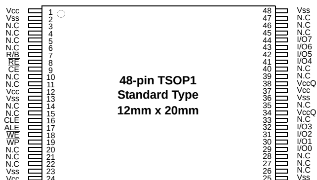
K9LBG08U0A-SCB0/SIB0
