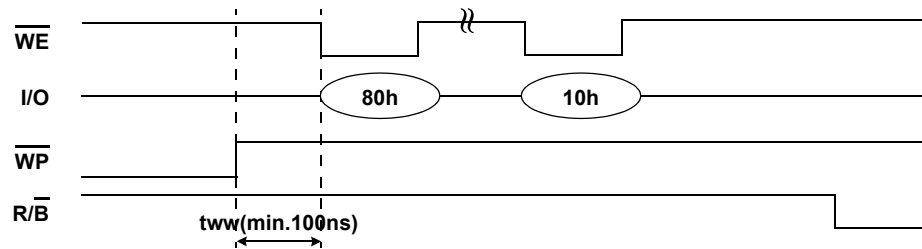
Figure C-1. Program Operation
