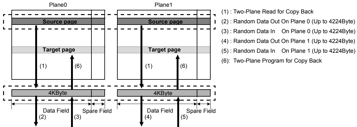
Figure B-4. 2-Plane Copy-Back Program Operation with Random Data Input
