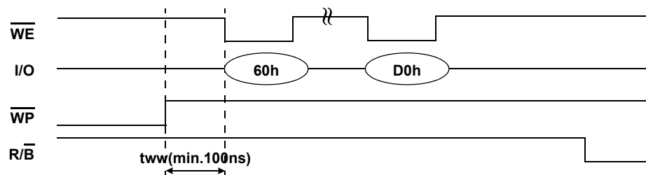
Figure C-2. Erase Operation
