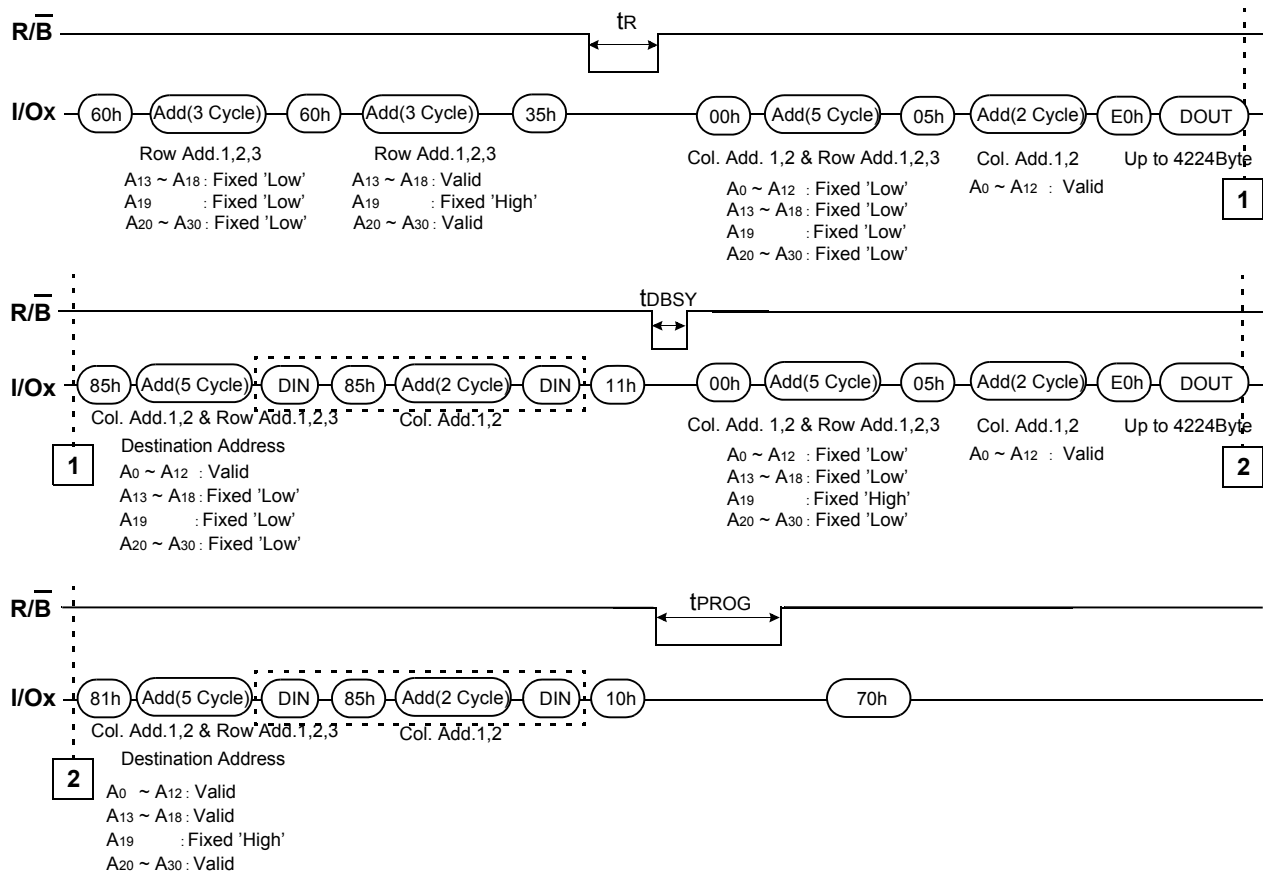
Figure B-4. 2-Plane Copy-Back Program Operation with Random Data Input
