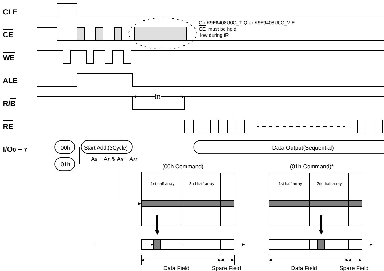
Figure 3. Read1 Operation
