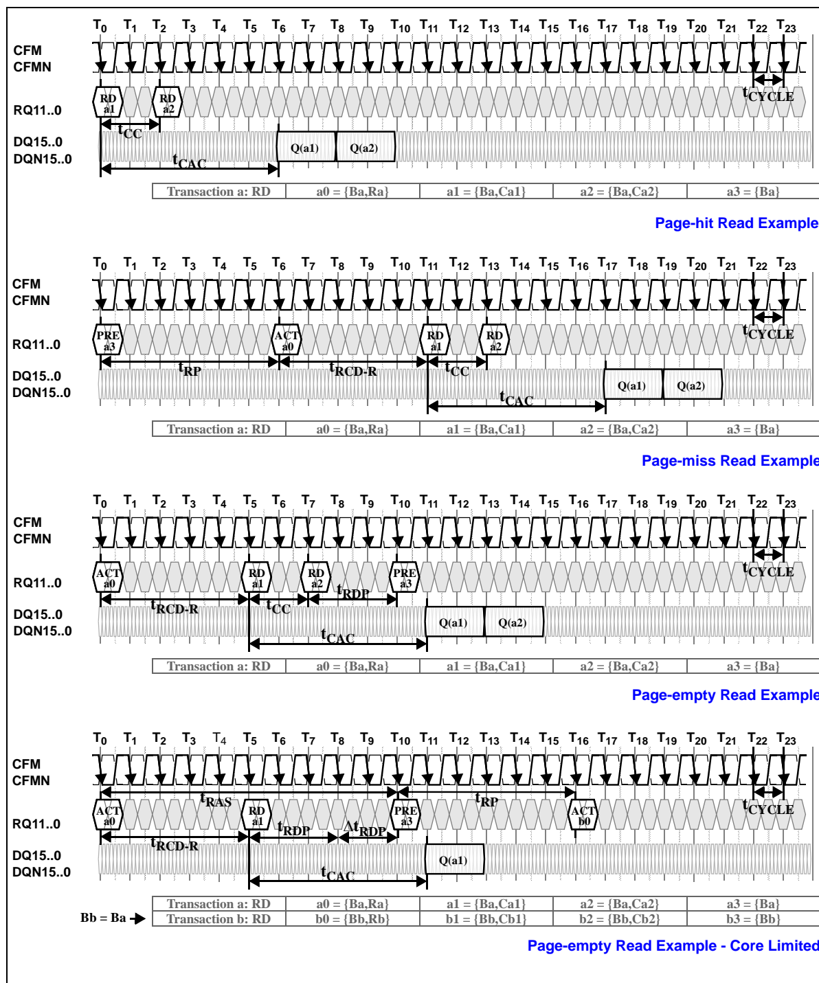
Figure 10 : Read Transactions
