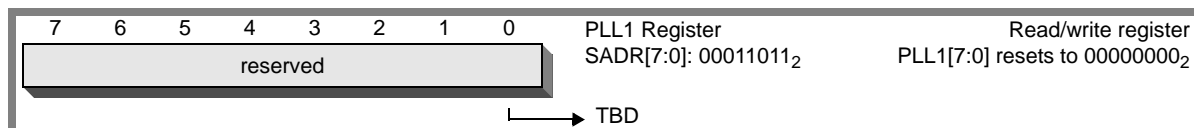
Figure 40 : IFT Register
