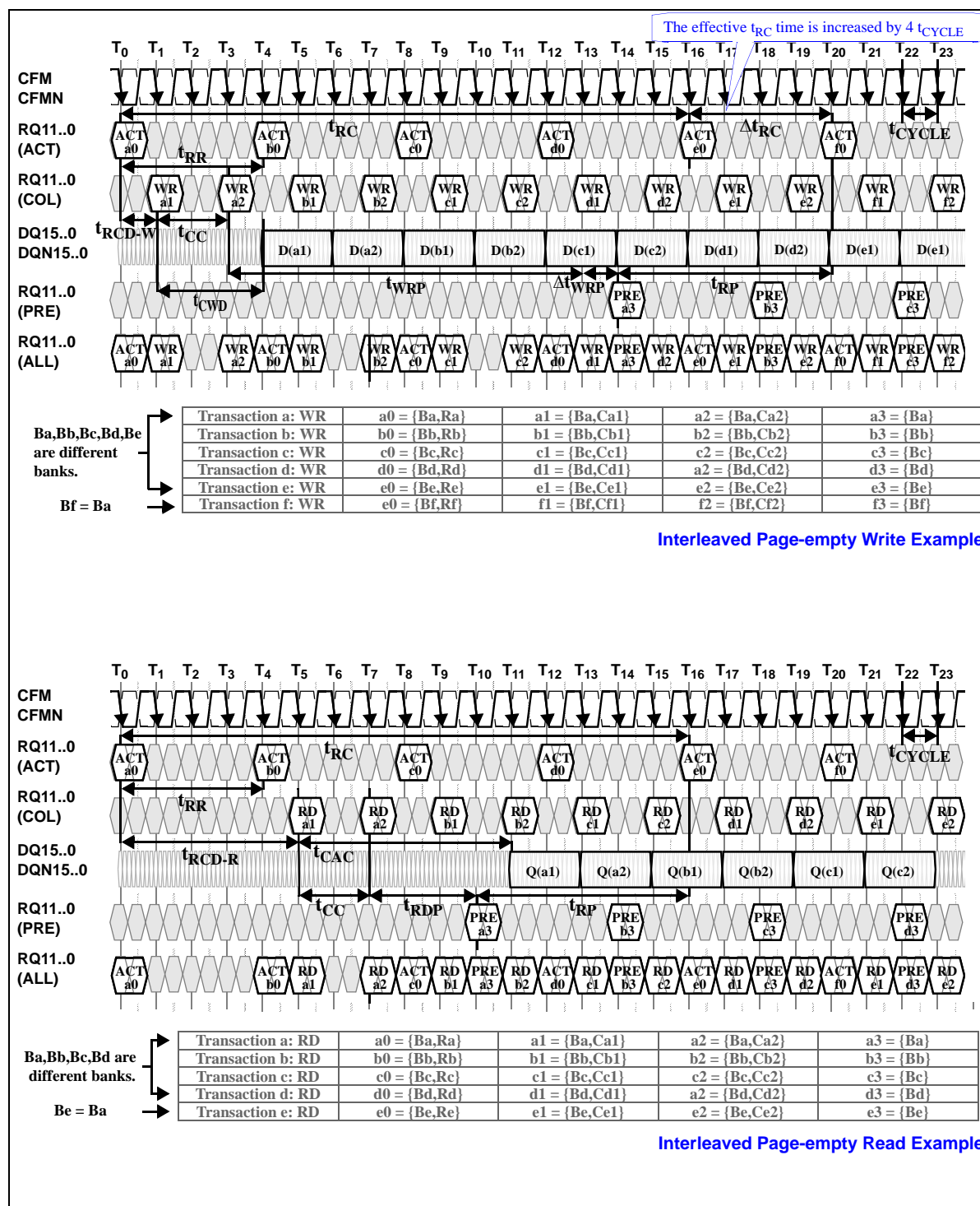
Figure 11 : Interleaved Transactions
