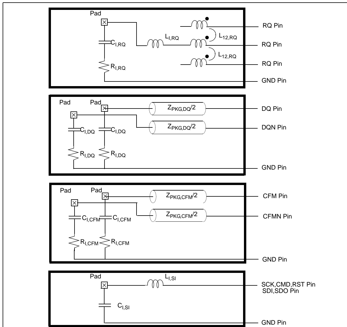
Figure 64 : Equivalent Circuits for Package Parasitic
