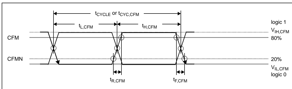
Figure 58 : Clocking Waveforms
