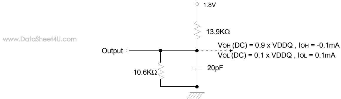
Figure 5. DC Output Load Circuit
