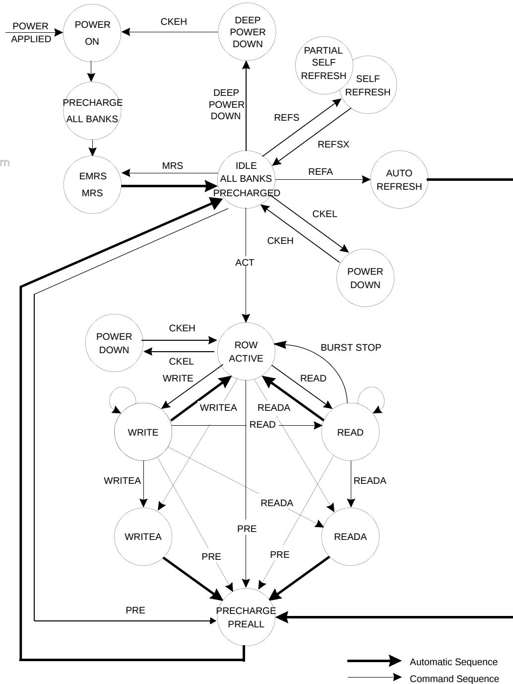
Figure.1 State diagram
