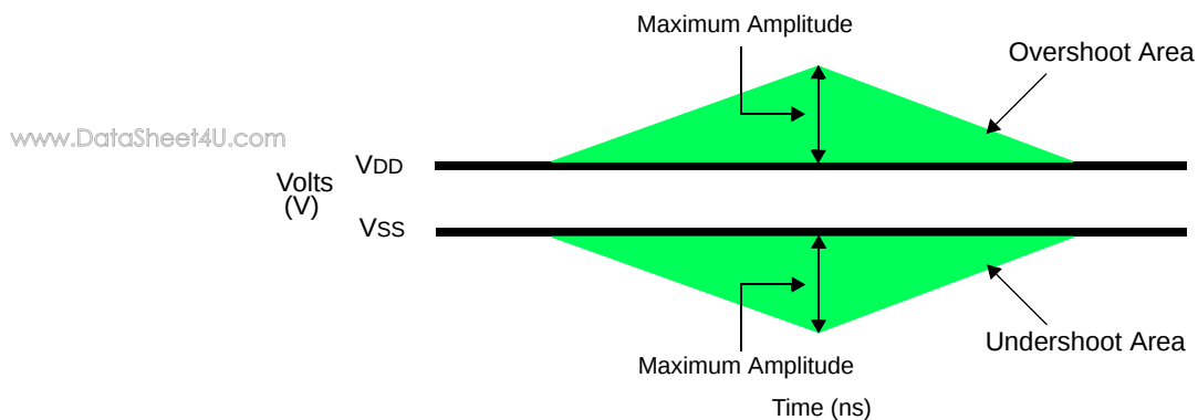
Figure.8 AC Overshoot and Undershoot Definition for Address and Control Pins
